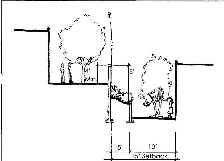
Grade Management over 8' change in Elevation
